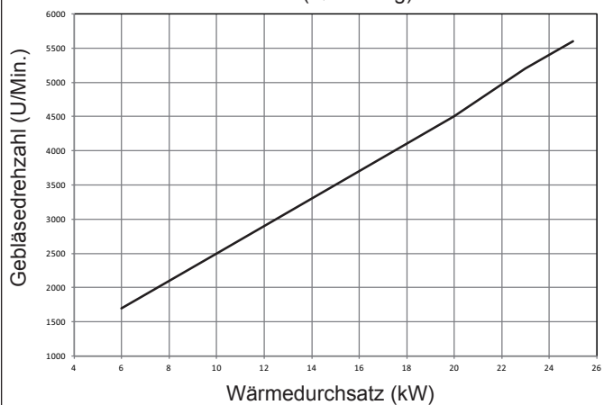
COs.a. Kurve (Qnheating)
