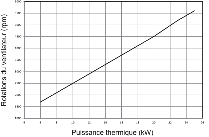
Courbe Cos.a. (Qnheating)
