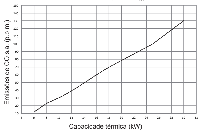
Curva COs.a. (Qnheating)
