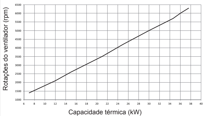
Curva HTG (Qnheating)
