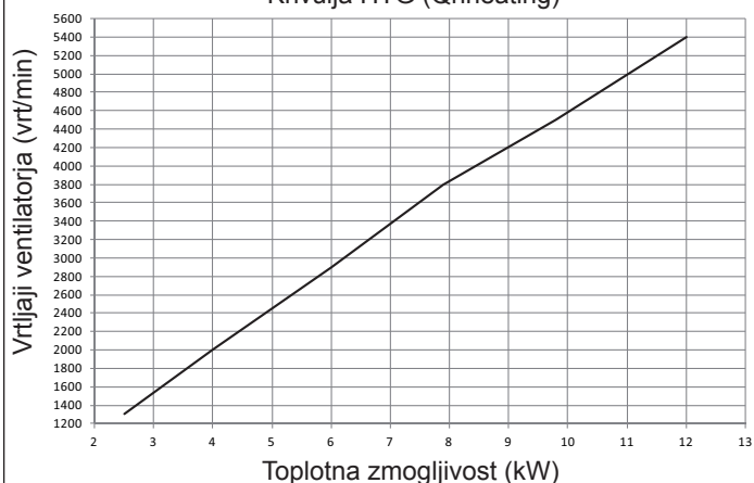
Krivulja HTG (Qnheating)
