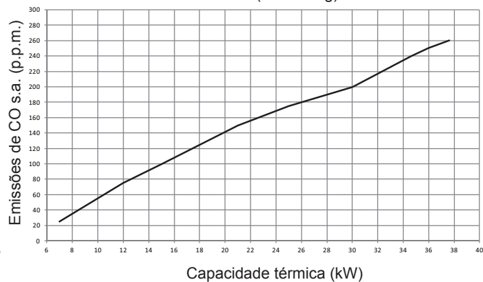
Curva COs.a. (Qnheating)
